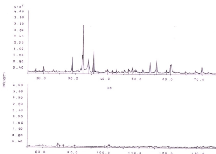
Figure. 1 : X-ray diffraction pattern of compound Y 1 Ca 0.5 Fe 3 Al 1 V 0.5 O 12
