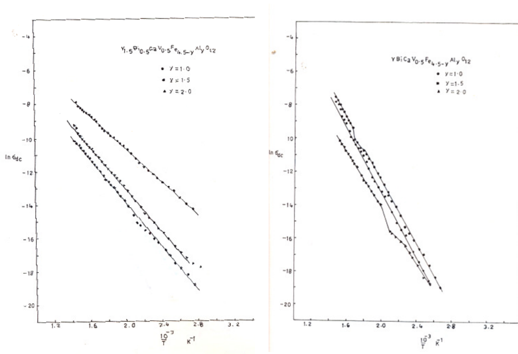
Figure 2: For Electrical Conductivity \ln \sigma verses 1/T \times 10^{-3} \text{ K}^{-1}
