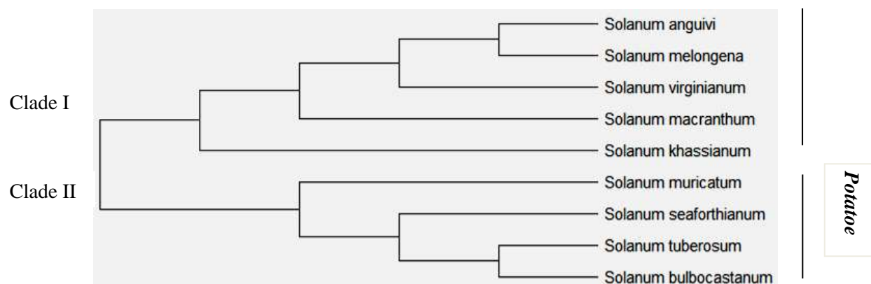
Figure 1: Phylogenetic tree of nine Solanum species based on maximum parsimony analysis based of trnL-F sequences
