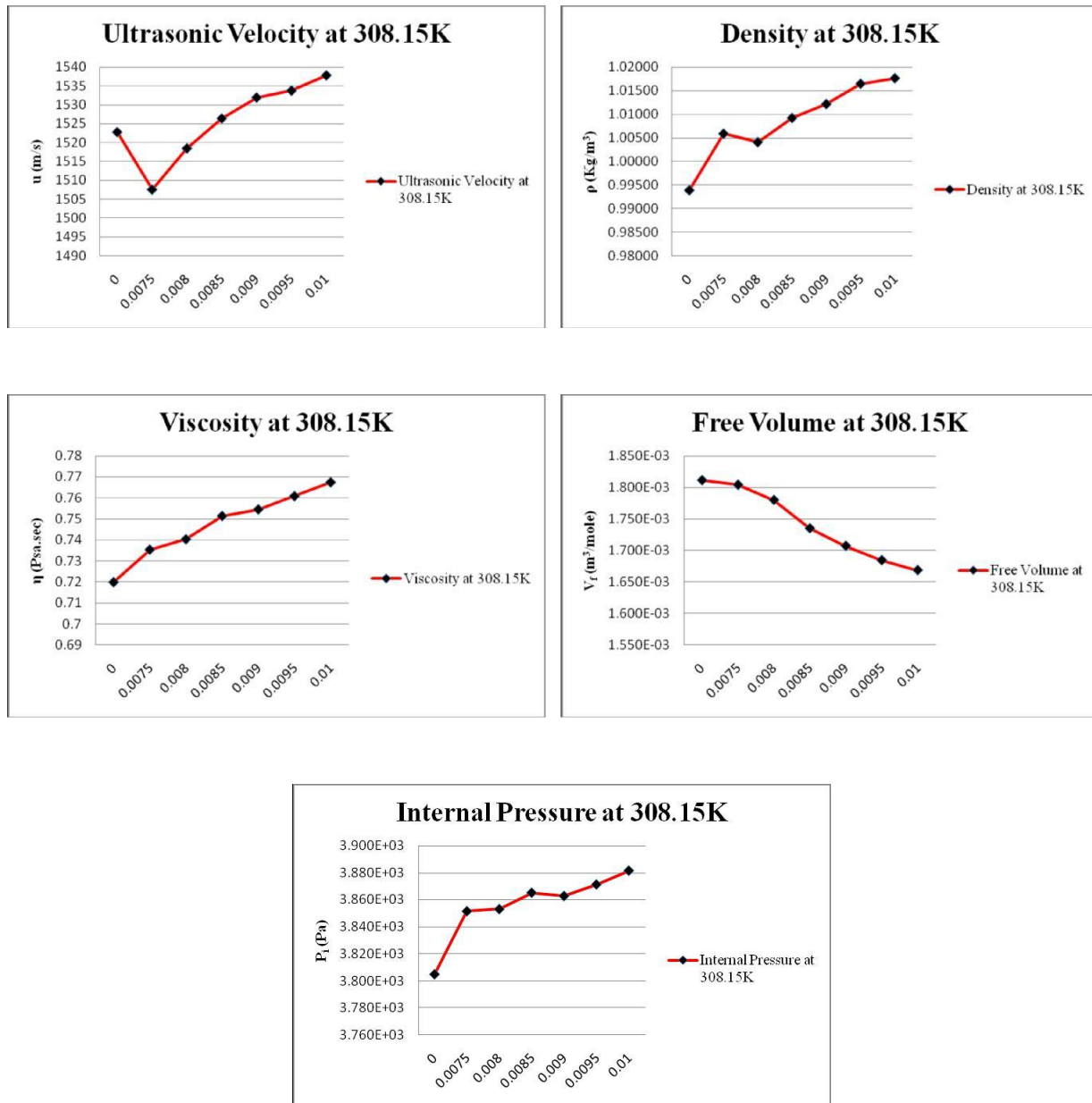
Fig 6: ultrasonic velocity, density, viscosity, free volume and Internal Pressure for aqueous L-Valine at 308.15K
