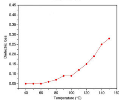
Fig (b) Temperature dependence of dielectric loss for ADP doped with 1 mol% of AmCl.
