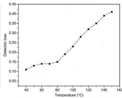
Fig (h) Temperature dependence of dielectric loss for pure ADP
