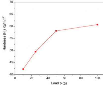
Fig (l) Vickers hardness plot of pure ADP
