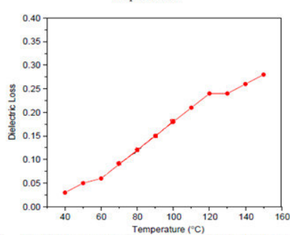
Fig (j) Temperature dependence of dielectric loss for ADP doped with 1 mol% of DML.
