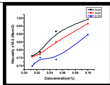
Fig. 4:-Variation of Viscosity with concentration and temperature
