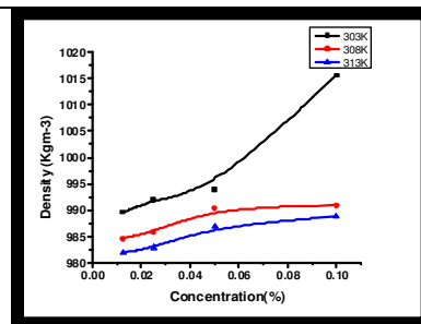
Fig. 2:-Variation of Density with concentration and temperature.
