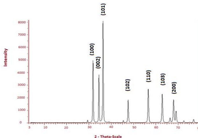
Figure 1. X Ray diffraction pattern of ZnO nanoparticles
