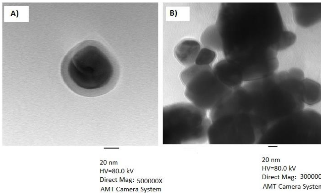
Figure 3. TEM images of ZnO nanoparticles showing regular and hexagonal morphology at 400°C.
