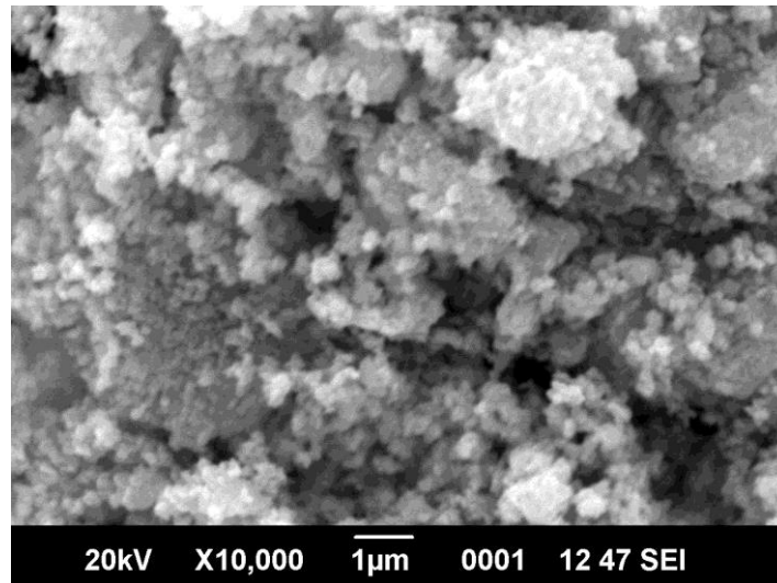
Figure 2 SEM characterization of ZnO nanoparticles confirming circular morphology and presence of overlapped nanoparticles.
