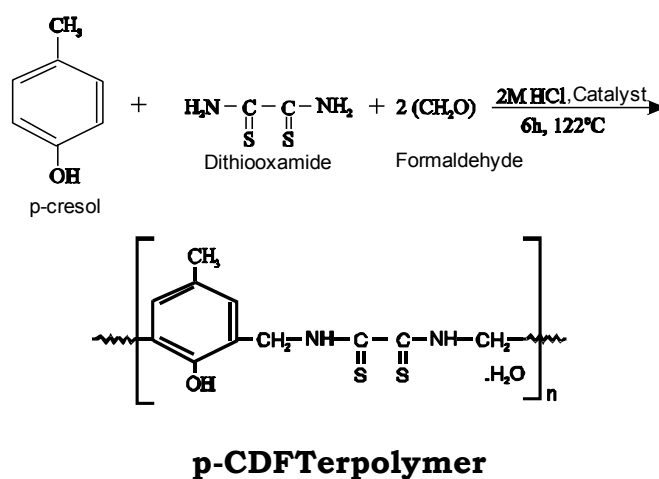
Fig. 1 Reaction and Suggested Structure of Representative p-CDF -I Terpolymer Resin
