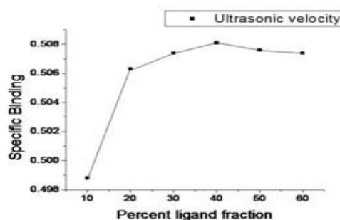
Figure 6 & 7: Ultrasonic velocity/ Specific binding Vs % ligand fraction at pH 5
