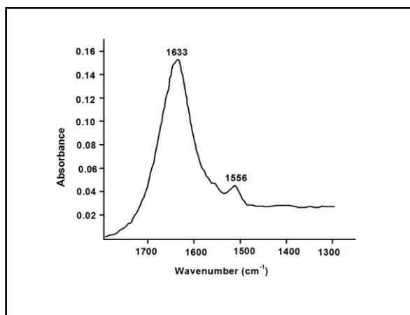
Fig: 8 FT-IR spectrum of BSA
