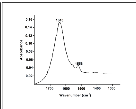
Fig: 9: FT-IR spectrum OF BSA-ligand complex
