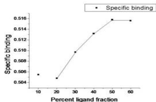
Figure 2 & 3: Ultrasonic velocity/ Specific binding Vs % ligand fraction at pH 3
