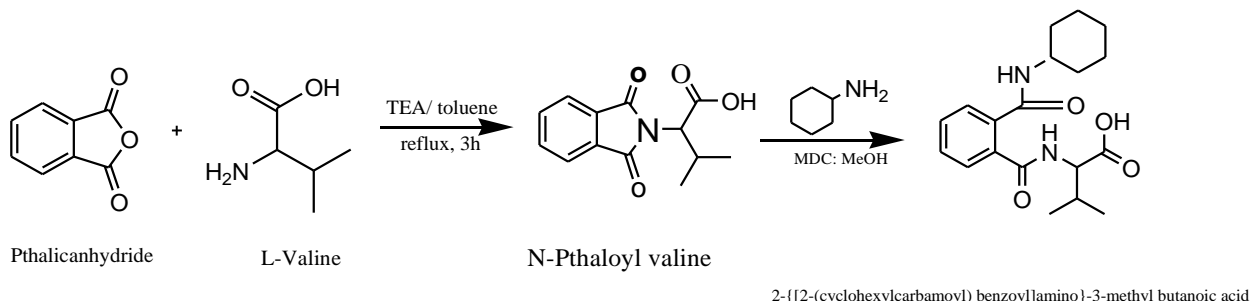
Figure 1: Scheme for the preparation of 2-[[2-(cyclohexylcarbamoyl) benzoyl]amino]-3-methyl butanoic acid
