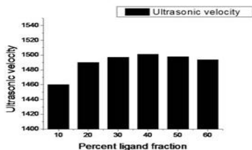
Figure 6 & 7: Ultrasonic velocity/ Specific binding Vs % ligand fraction at pH 5
