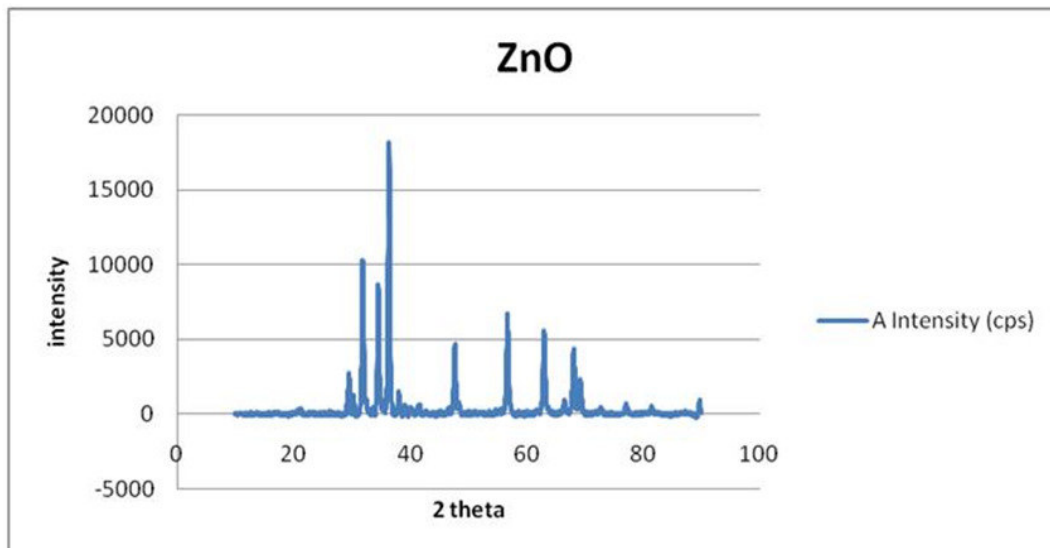
Fig. 3: XRD pattern of the synthesized ZnO nanostructures
