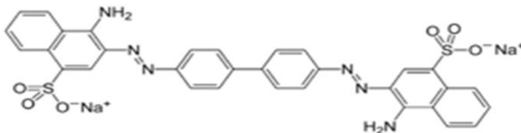
Fig 1: Chemical structure of congo red (CR)dye
