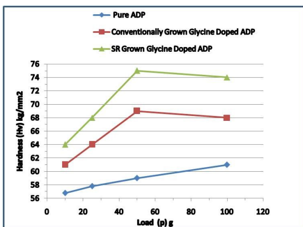
Fig. 2. Vicker's microhardness of grown crystals
