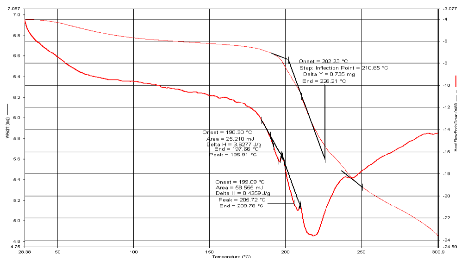
Fig.5. TG/DTA spectra of glycine doped ADP crystal
