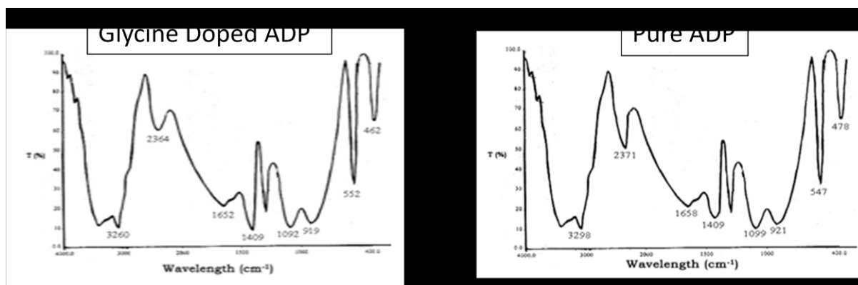
Fig.4. FTIR spectrum of pure and glycine doped ADP
