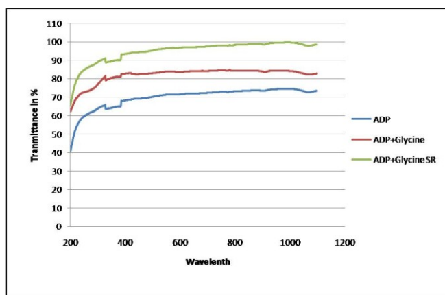
Fig. 3. UV-Vis transmission spectra of pure and doped ADP crystals
