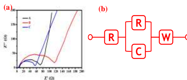
Fig. 3 - Electrochemical impedance study of NiO thin film, (a) Nyquist plot NiO Nanoflex, (b) equivalent circuit diagram
