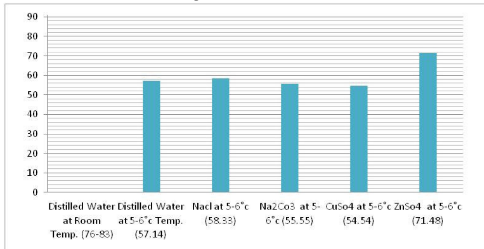
Series graph: Showing urea excretion in earthworm P.posthuma in cold stressed and toxic solutions.
