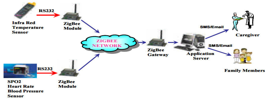
Fig. 1: Homecare System Architecture
